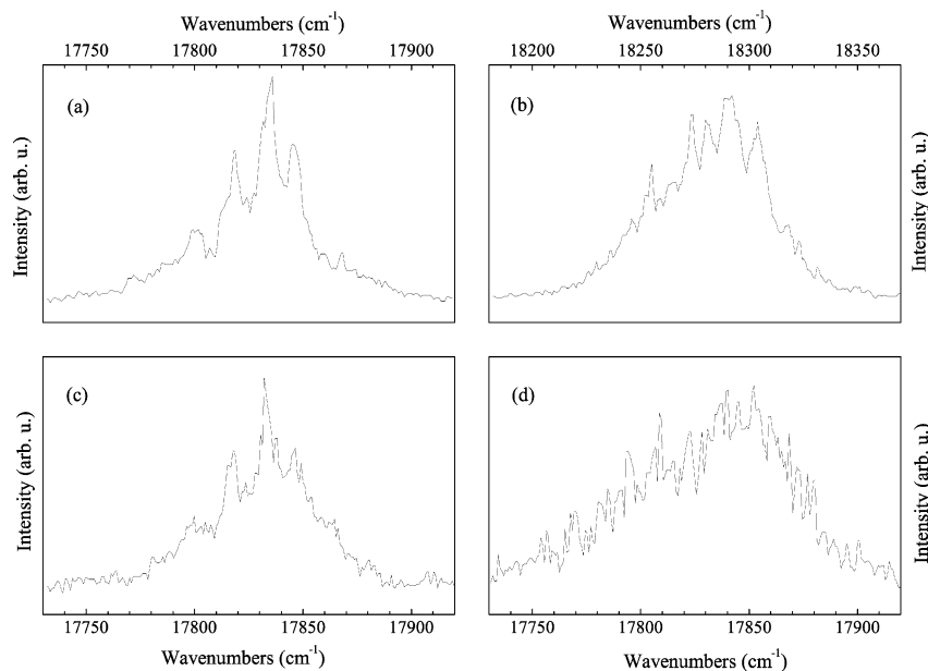
Figure 5. Close-ups of various bands of the \tilde{C} \leftarrow \tilde{X} photodissociation spectra of the C_8H_6^+ - Ar_{1,2} ionic complexes taken in various conditions. (a) Origin of the electronic transition measured in the C_8H_6^+ - Ar cation prepared via a two-color scheme via the 0(S_1) intermediate state, i.e., prepared in the vibrationless level of the electronic ground state. (b) Band 13_0^1 in the same conditions as (a). (c) Region of the origin of the electronic transition measured with the cation prepared in its 35_1 vibrationally excited state in the electronic ground state. (d) Origin band of the C_8H_6^+ - Ar_2 prepared in a one-color scheme.
